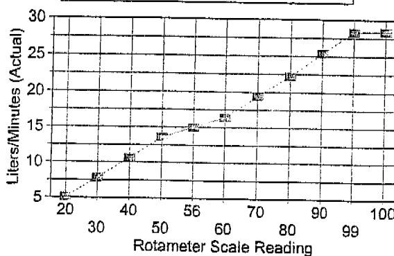
ROTAMETER CALIBRATION Calibrated 02/11/02 - HV-21
